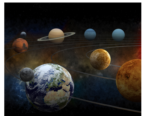
planets
