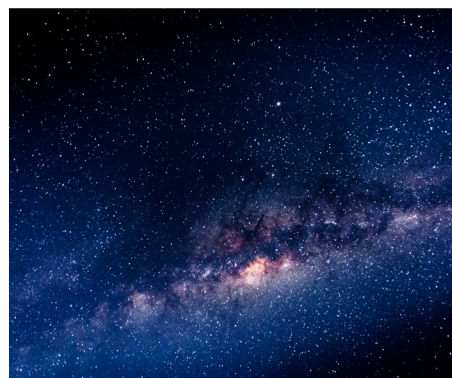
stars
