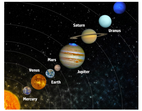
planets
