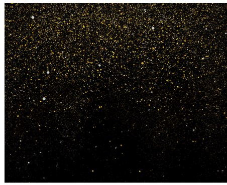
stars
