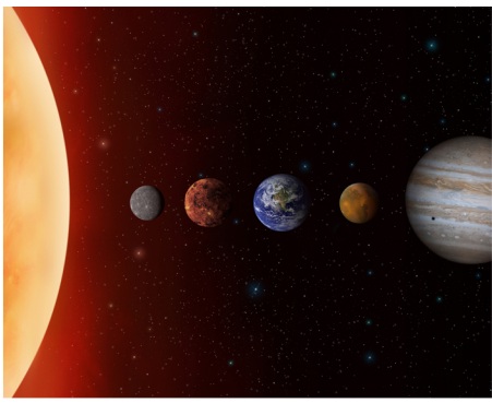
astronomy
