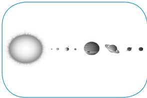
solar system
